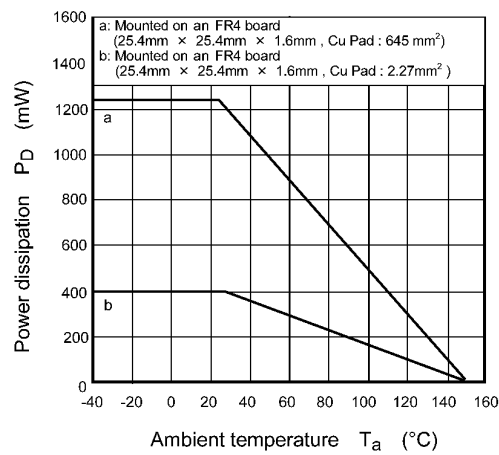
Fig. 8.15 P_D - T_a
