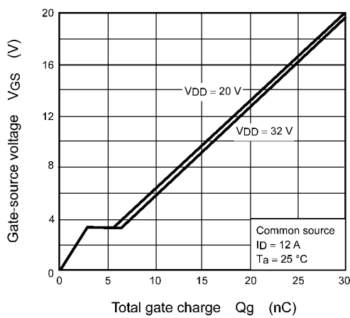
Fig. 8.11 Dynamic Input Characteristics
