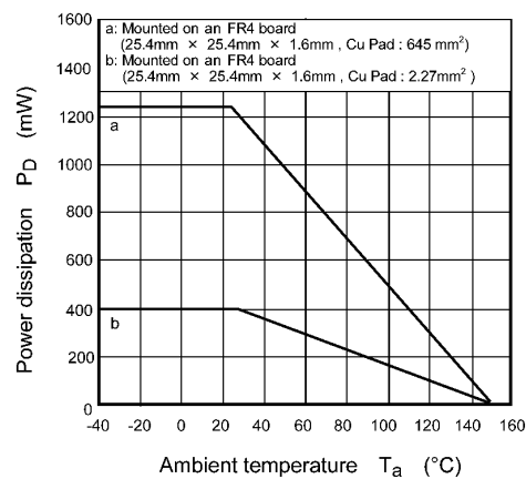
Fig. 8.13 P_D - T_a
