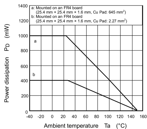
Fig. 8.12 P_D - T_a
