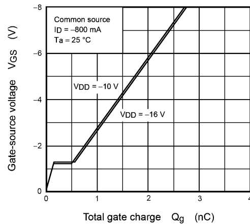
Fig. 7.12 Dynamic Input Characteristics
