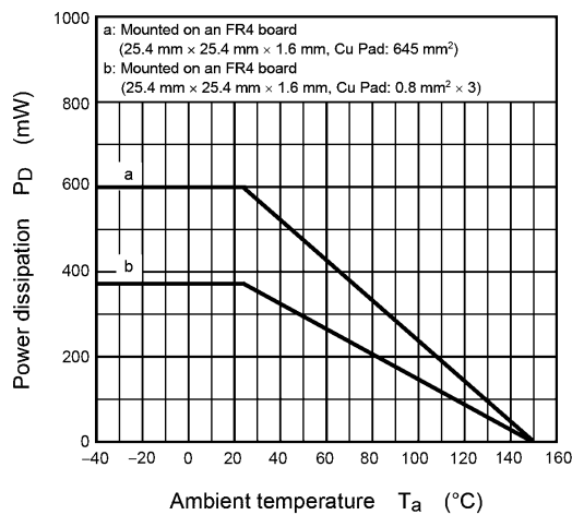
Fig. 8.13 P_D - T_a
