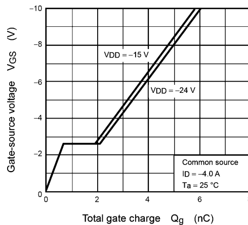
Fig. 8.12 Dynamic Input Characteristic
