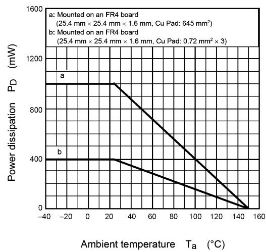
Fig. 8.14 P_D - T_a
