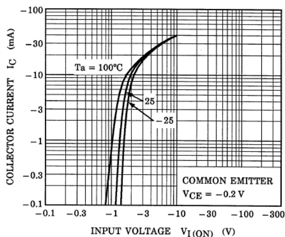
Fig. 10.1 RN2907 I_C - V_{I(ON)}
