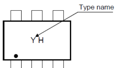
Fig. 9.1 Marking RN2907FE
