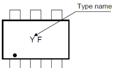
Fig. 9.6 Marking RN2906FE
