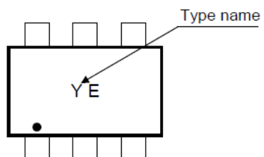
Fig. 9.5 Marking RN2905FE
