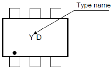
Fig. 9.4 Marking RN2904FE
