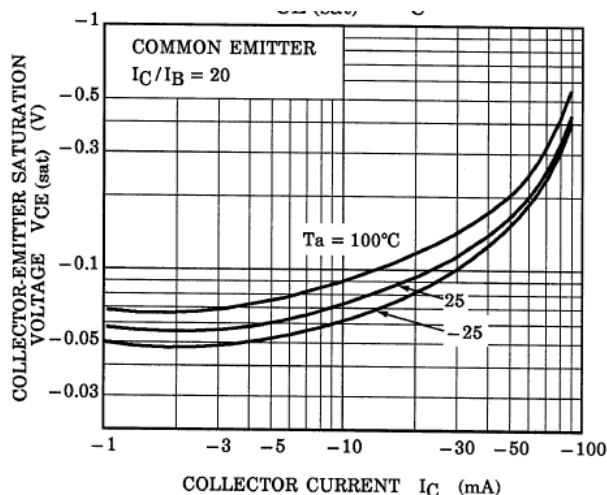
Fig. 10.24 RN1206 V_{CE(sat)}-I_C
