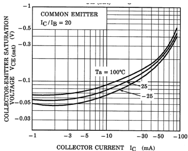
Fig. 10.23 RN2905 V_{CE(sat)}-I_C
