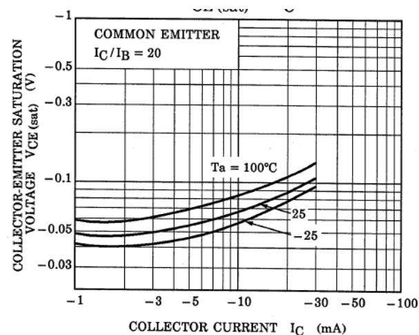
Fig. 10.22 RN2904FE V_{CE(sat)}-I_C
