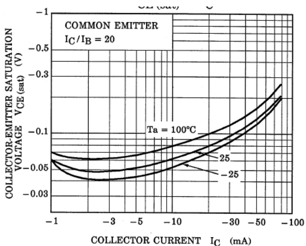
Fig. 10.21 RN2903FE V_{CE(sat)}-I_C
