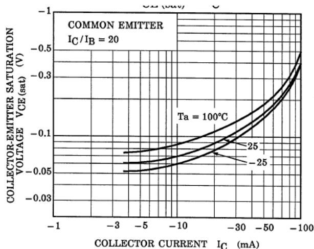
Fig. 10.20 RN2902FE V_{CE(sat)}-I_C
