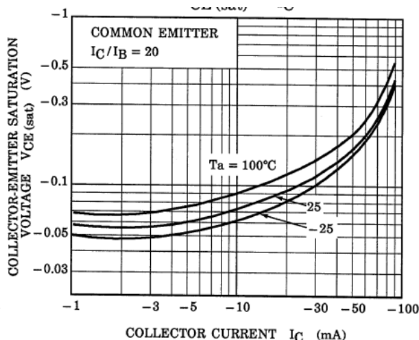
Fig. 10.24 RN2906FE V_{CE(sat)}-I_C
