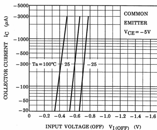
Fig. 9.15 RN2425 I_C - V_{I(OFF)}
