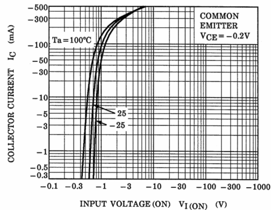
Fig. 9.14 RN2426 I_C - V_{I(ON)}
