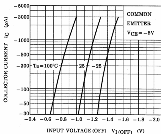
Fig. 9.9 RN2423 I_C - V_{I(OFF)}
