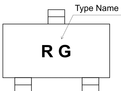
Fig. 8.7 Marking RN2427
