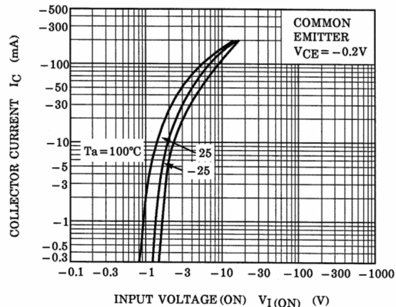
Fig. 9.8 RN2424 I_C - V_{I(ON)}
