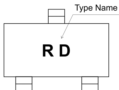
Fig. 8.4 Marking RN2424
