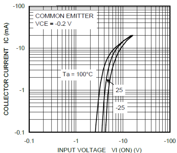
Fig. 10.5 RN2318 I_C - V_{I(ON)}
