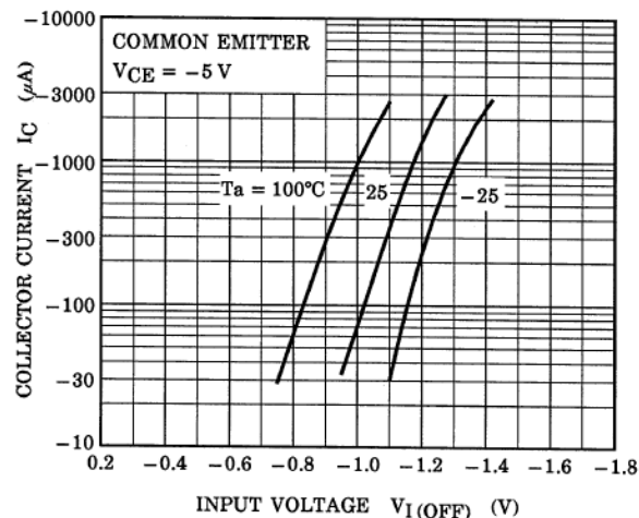
Fig. 10.4 RN2107 I_C - V_{I(OFF)}
