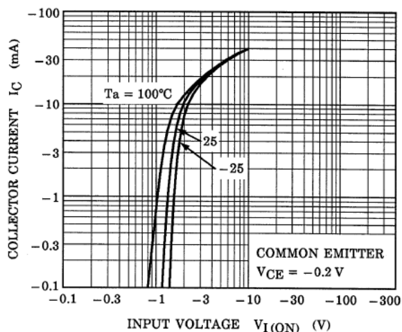
Fig. 10.1 RN2107 I_C - V_{I(ON)}
