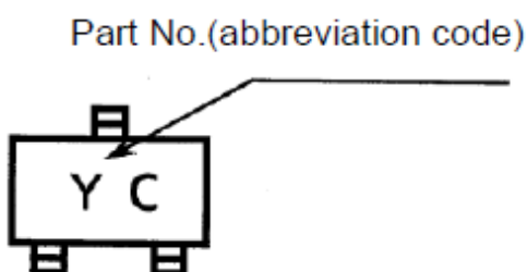
Fig. 9.3 Marking RN2103
