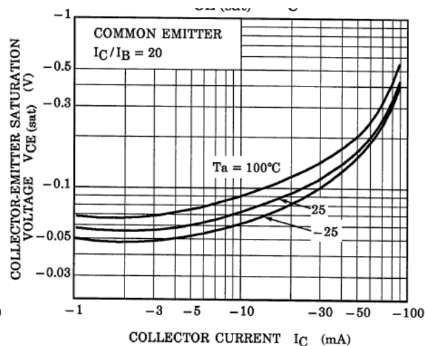
Fig. 10.24 RN2106 V_{CE(sat)}-I_C
