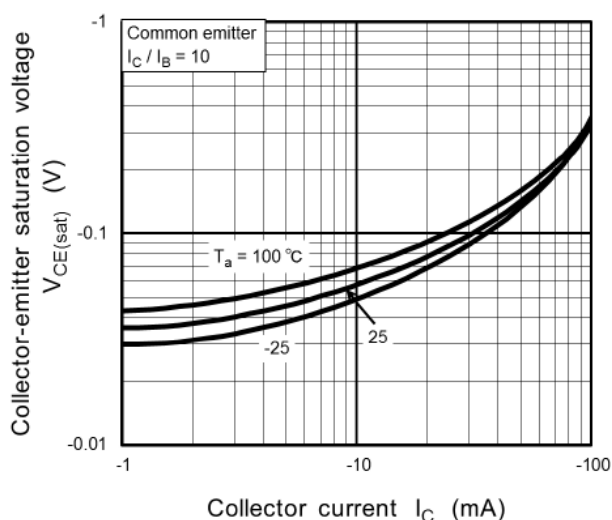
Fig. 11.23 RN2105MFV V_{CE(sat)}-I_C
