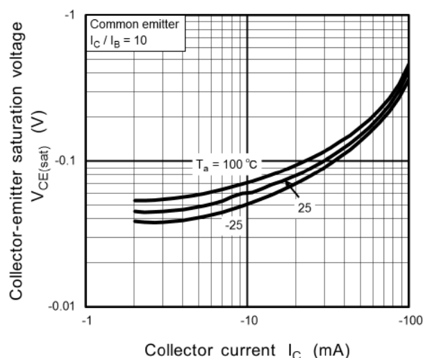
Fig. 11.20 RN2102MFV V_{CE(sat)}-I_C
