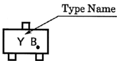
Fig. 10.2 Marking RN2102MFV
