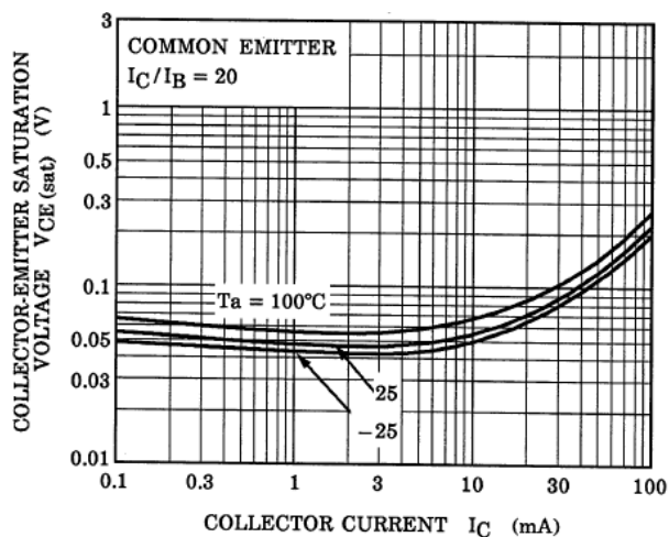
Fig. 9.8 RN1911 V_{CE(sat)}-I_C
