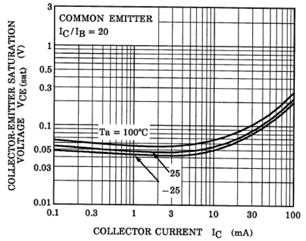
Fig. 9.8 RN1911 V_{CE(sat)}-I_C
