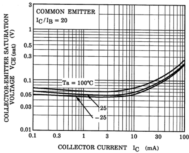
Fig. 9.7 RN1910 V_{CE(sat)}-I_C
