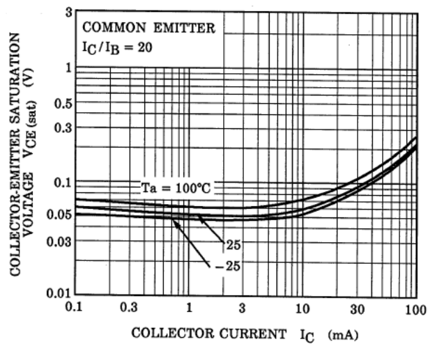
Fig. 9.7 RN1910 V_{CE(sat)}-I_C
