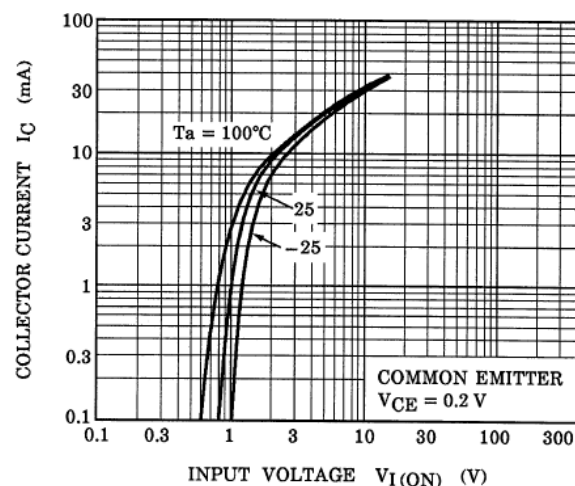
Fig. 10.2 RN1908 I_C - V_{I(ON)}
