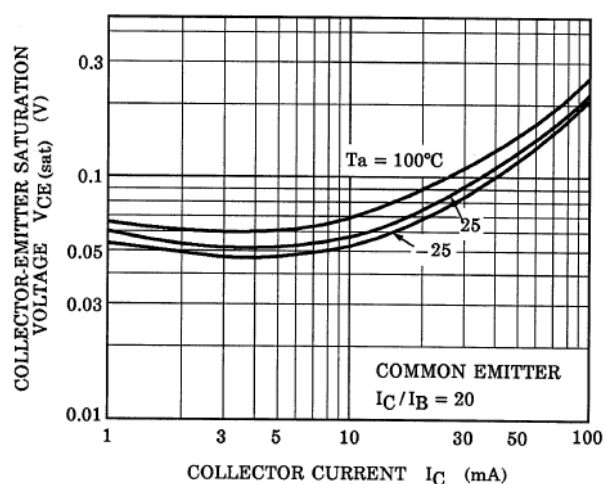
Fig. 10.23 RN1905 V_{CE(sat)}-I_C
