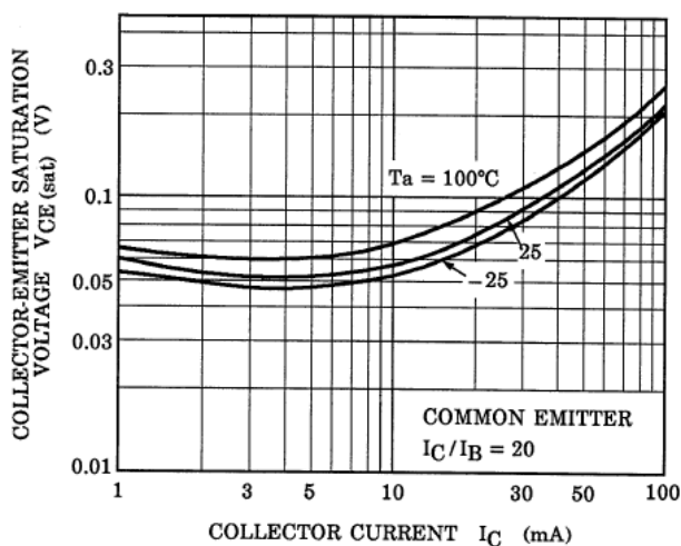
Fig. 10.23 RN1905FE V_{CE(sat)}-I_C
