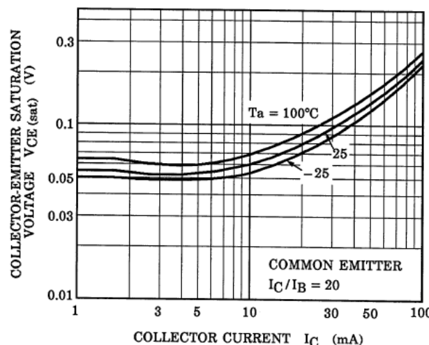
Fig. 10.24 RN1406 V_{CE(sat)}-I_C
