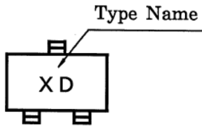
Fig. 9.4 Marking RN1404
