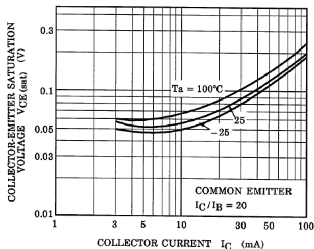
Fig. 10.20 RN1402 V_{CE(sat)}-I_C
