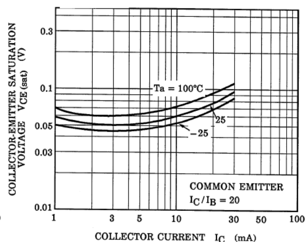
Fig. 10.22 RN1404 V_{CE(sat)}-I_C
