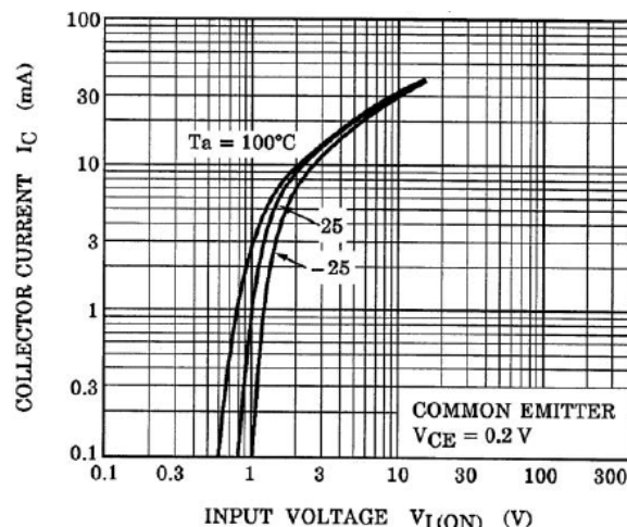
Fig. 10.2 RN1308 I_C - V_{I(ON)}
