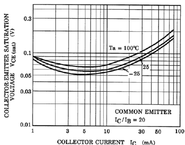
Fig. 10.21 RN1303 V_{CE(sat)}-I_C
