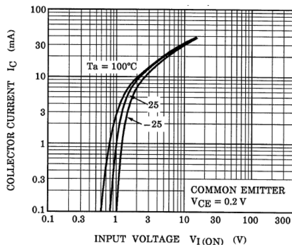
Fig. 10.2 RN1108 I_C - V_{I(ON)}
