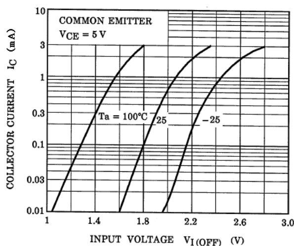
Fig. 10.6 RN1109 I_C - V_{I(OFF)}
