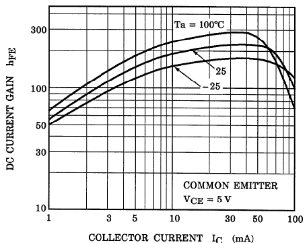
Fig. 10.7 RN1107 h_{FE} - I_C
