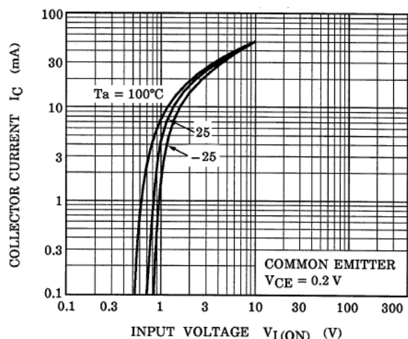
Fig. 10.1 RN1107 I_C - V_{I(ON)}
