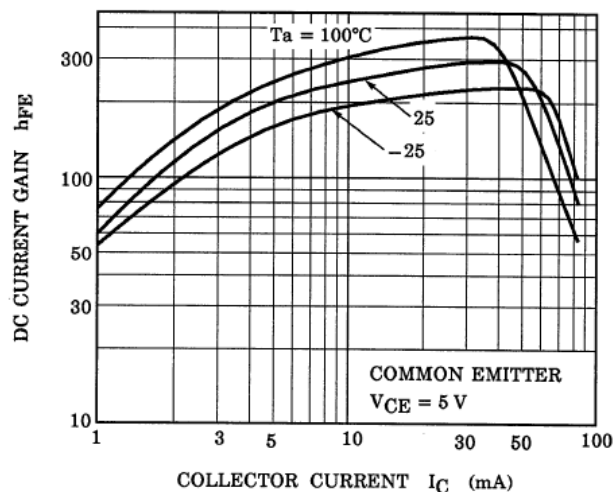
Fig. 10.8 RN1108 h_{FE} - I_C
