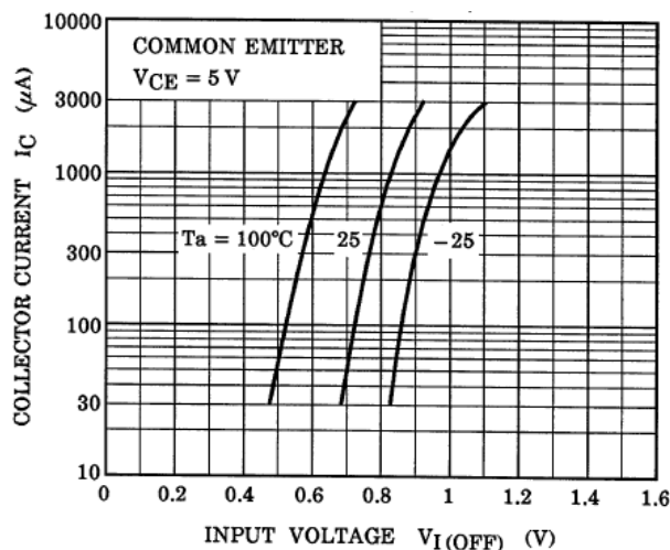
Fig. 10.4 RN1107 I_C - V_{I(OFF)}
