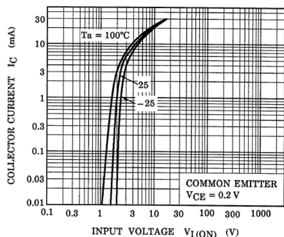
Fig. 10.3 RN1109 I_C - V_{I(ON)}
