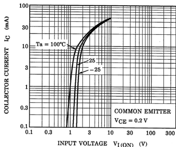
Fig. 10.2 RN1102 I_C - V_{I(ON)}
