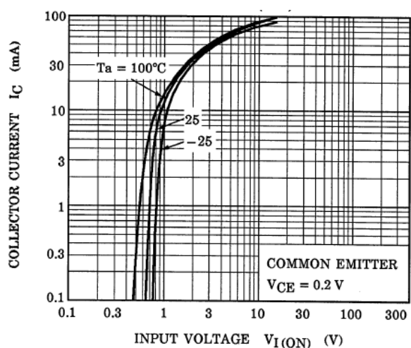
Fig. 10.5 RN1105 I_C - V_{I(ON)}
