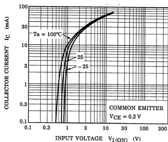
Fig. 10.6 RN1106 I_C - V_{I(ON)}
