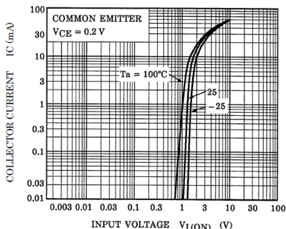
Fig. 10.1 RN1101 I_C - V_{I(ON)}
