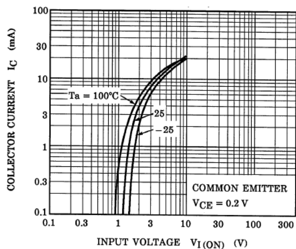
Fig. 10.4 RN1104 I_C - V_{I(ON)}
