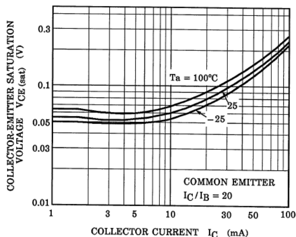
Fig. 10.24 RN1106 V_{CE(sat)}-I_C
