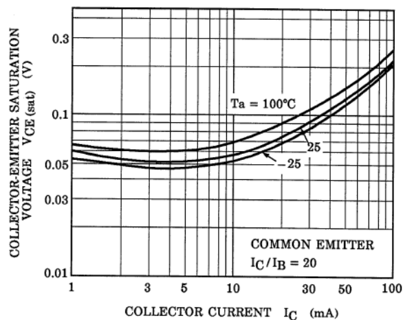
Fig. 10.23 RN1105 V_{CE(sat)}-I_C
