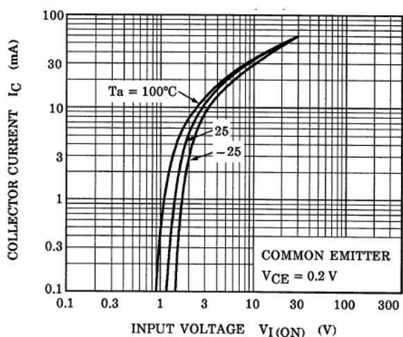
Fig. 10.3 RN1103 I_C - V_{I(ON)}
