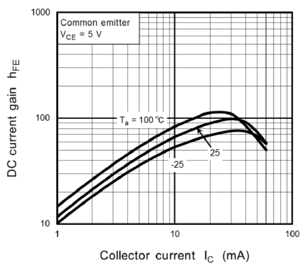
Fig. 11.14 RN1102MFV h_{FE} - I_C
