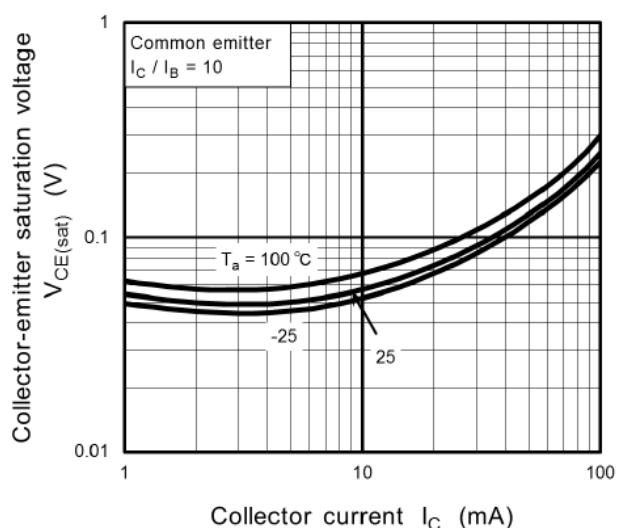
Fig. 11.23 RN1105MFV V_{CE(sat)}-I_C
