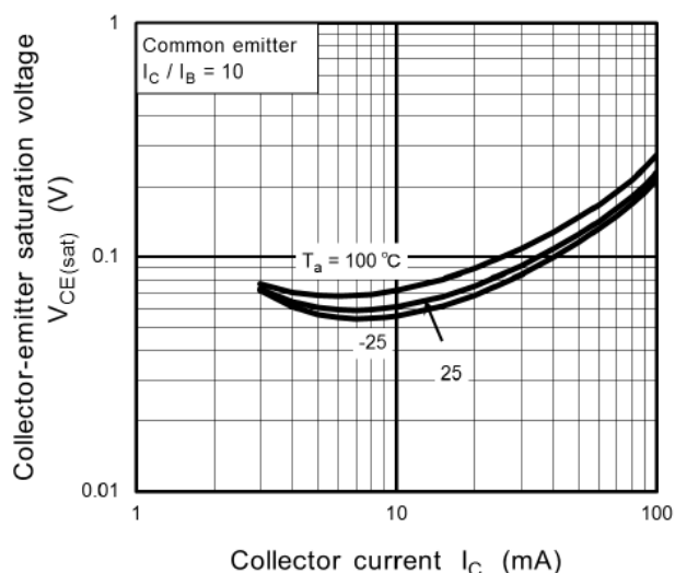
Fig. 11.19 RN1101MFV V_{CE(sat)}-I_C
