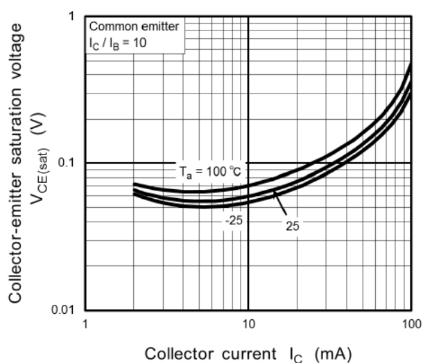
Fig. 11.20 RN1102MFV V_{CE(sat)}-I_C
