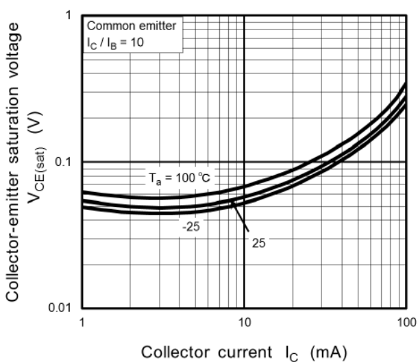
Fig. 11.24 RN1106MFV V_{CE(sat)}-I_C
