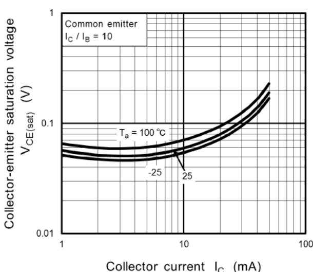
Fig. 11.22 RN1104MFV V_{CE(sat)}-I_C
