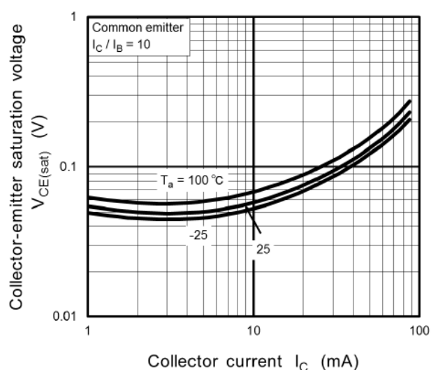
Fig. 11.21 RN1103MFV V_{CE(sat)}-I_C
