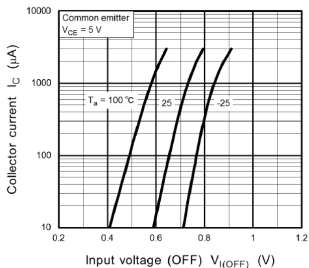
Fig. 11.11 RN1105MFV I_C - V_{I(OFF)}
