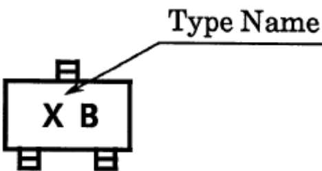
Fig. 9.2 Marking RN1102
