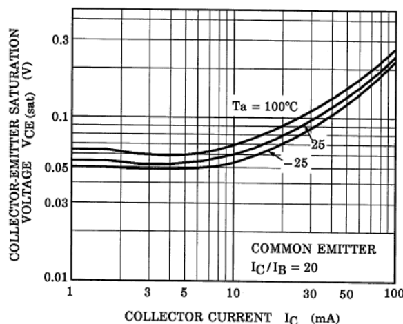
Fig. 10.24 RN1106 V_{CE(sat)}-I_C
