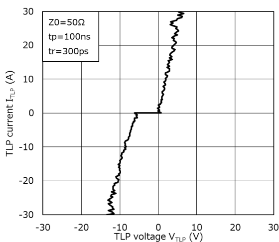
I_{TLP} - V_{TLP}
