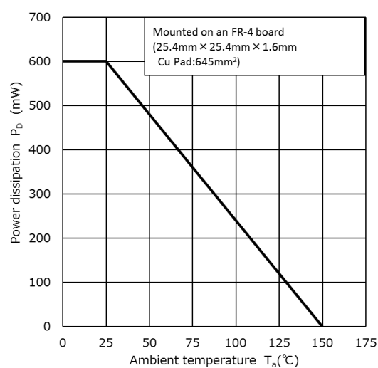
P_D - T_a
