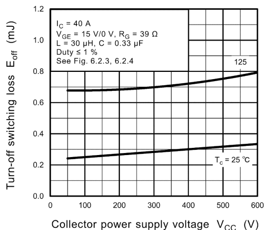
Fig. 8.14 E_{off} - V_{CC}
