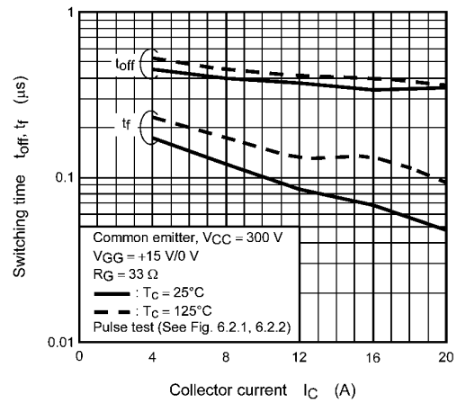
Fig. 8.10 t_{off}, t_f, t_d(off) - I_C
