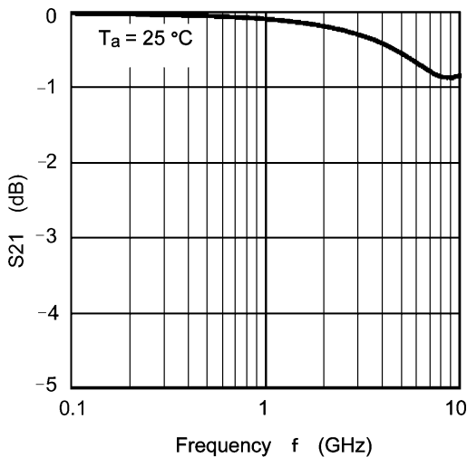
Fig. 9.5 S_{21} - f
