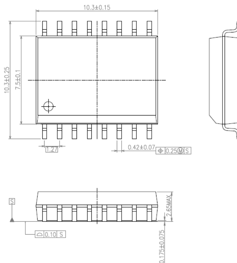
Figure 13.1 Package Dimensions
