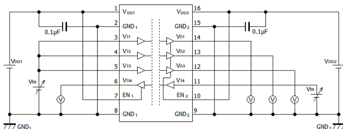
Fig. 12-7: DCL541L01/DCL541H01 V_{IH}/V_{IL} Test Circuit
