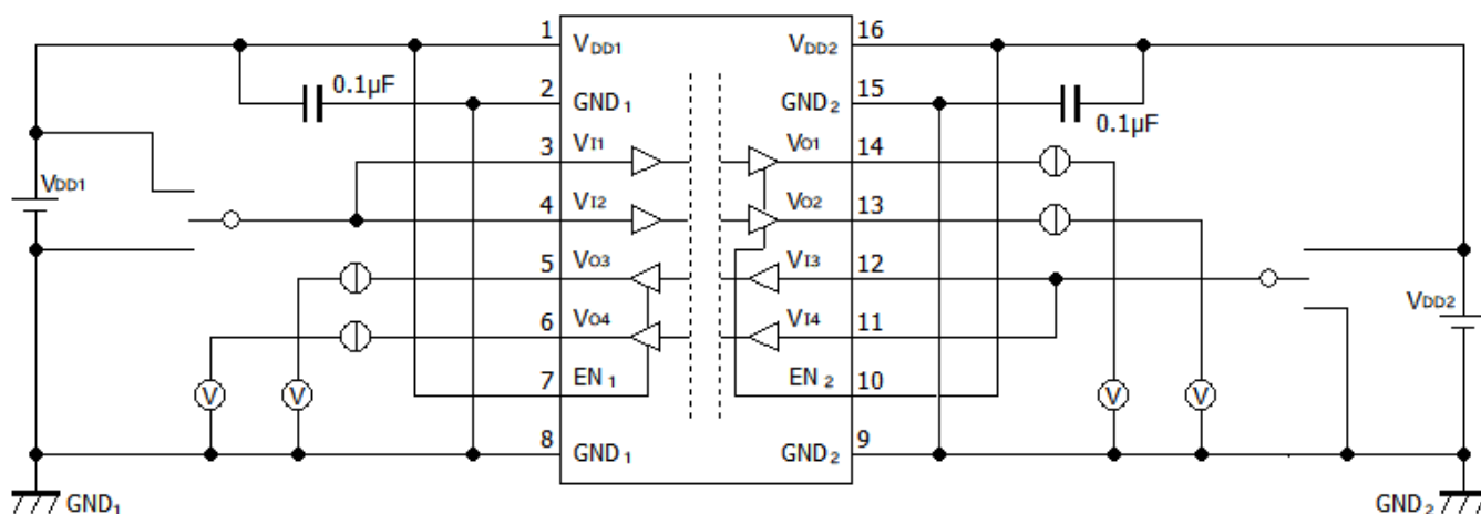
Fig. 12-6: DCL542L01/DCL542H01 V_{OH}/V_{OL} Test Circuit
