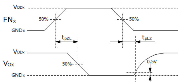
Fig. 12-14: DCL54xL01/DCL54xH01 Enable Propagation Delay Time Waveforms
