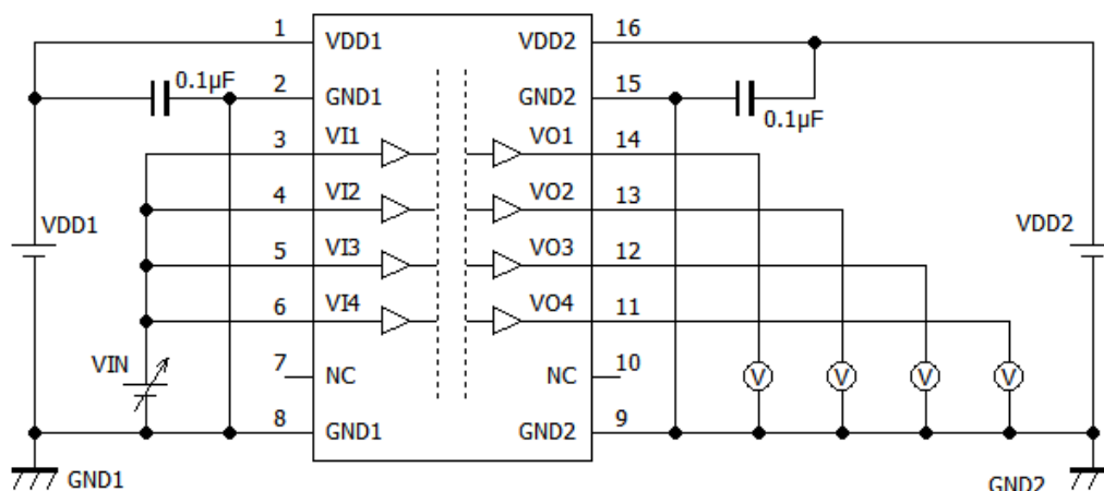
Fig.12-3-1. DCL540C01/DCL540D01 VIH/VIL Test Circuit
