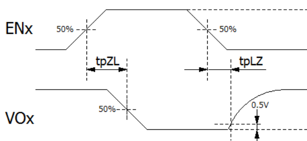
Fig.12-5. DCL540L01/ DCL540H01 Enable Propagation Delay Time Test Circuit and Waveforms
