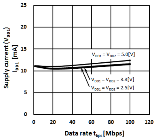
Fig.13-1. DCL540xx01 I_{DD1} Supply Current—Data rate
