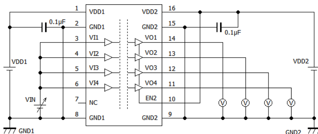
Fig.12-3-2. DCL540L01/DCL540H01 VIH/VIL Test Circuit
