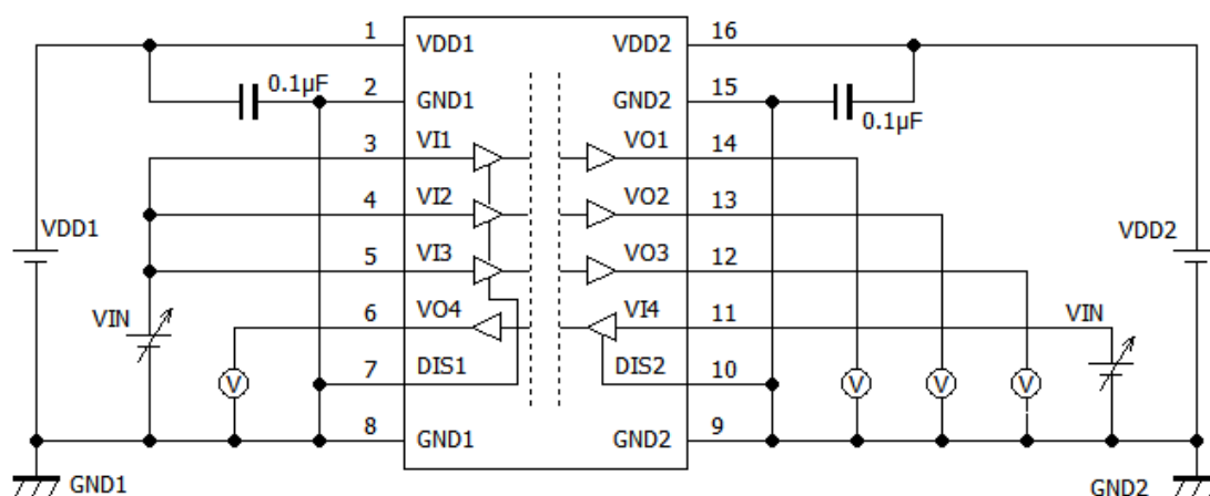
Fig.12-3-3. DCL541A01/DCL541B01 VIH/VIL Test Circuit
