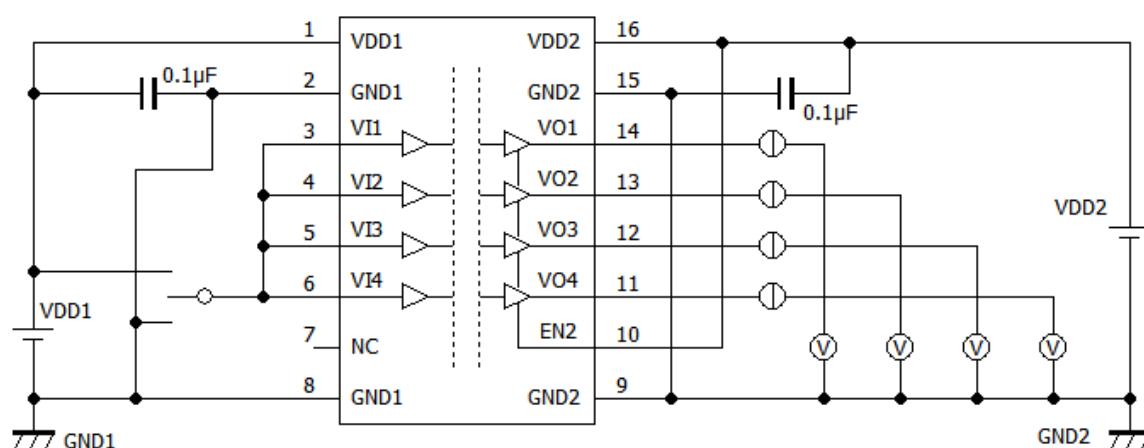
Fig.12-2-2. DCL540L01/DCL540H01 VOH/VOL Test Circuit
