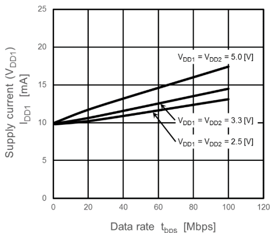
Fig.13-3. DCL541xx01 I_{DD1} Supply Current—Data rate
