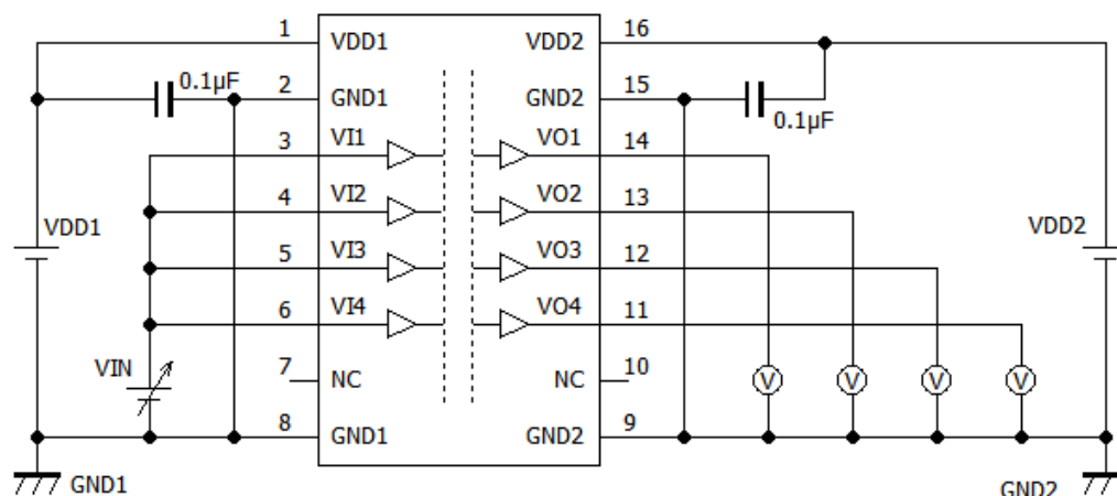
Fig.12-3-1. DCL540C01/DCL540D01 VIH/VIL Test Circuit
