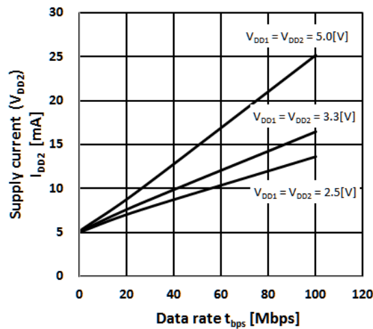
Fig.13.2. DCL540xx01 I_{DD2} Supply Current - Data rate
