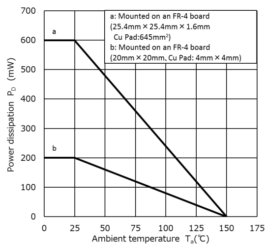
P_D - T_a
