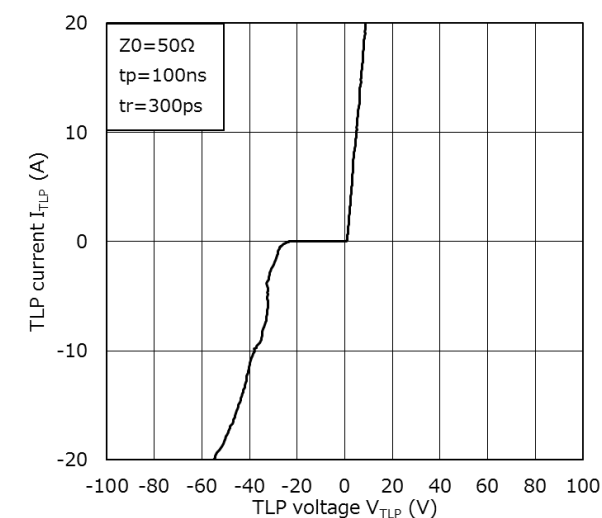
I_{TLP} - V_{TLP}
