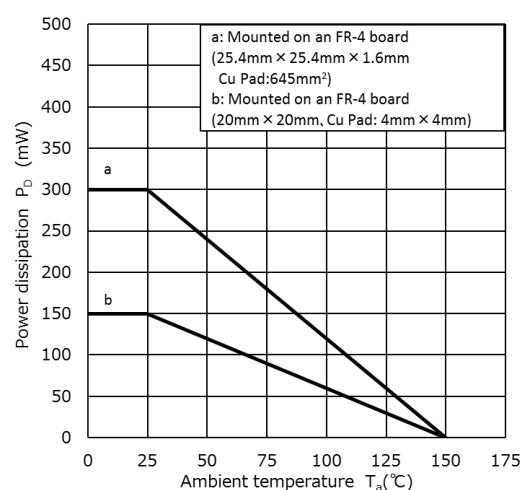
P_D - T_a
