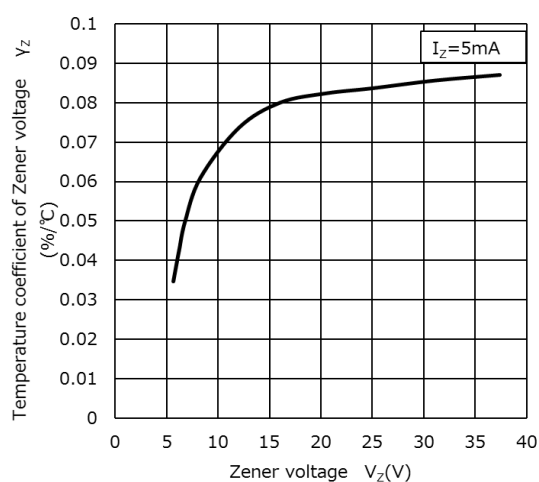
\gamma_Z - V_Z
