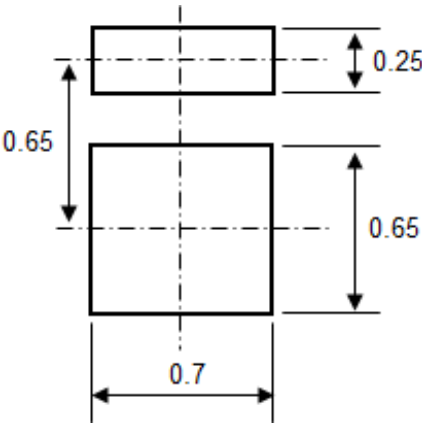
Fig. 7.1 Land Pattern Dimensions for Reference Only (Unit: mm)
