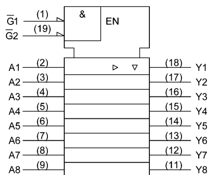
74VHC541FT
